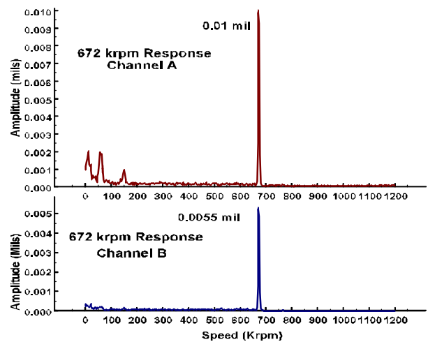
Fig 8. Spectrum for rotor at 672,000 rpm
