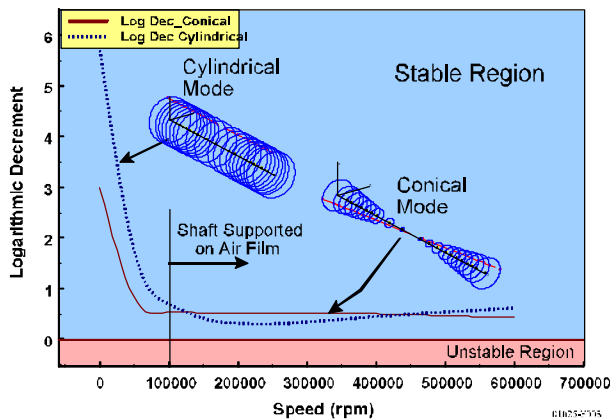
Fig 7. Stability map showing logarithmic decrement versus rotor speed for the rigid body natural frequencies
