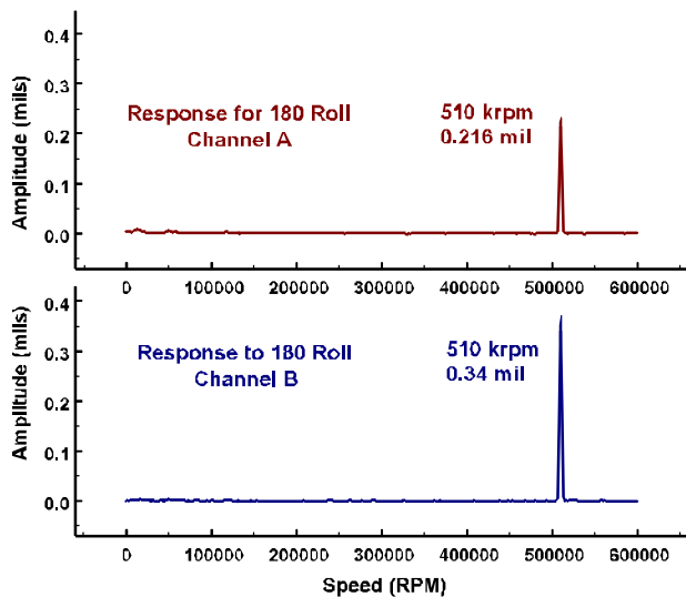
Fig. 11. Spectrum for 180° roll about spin axis
