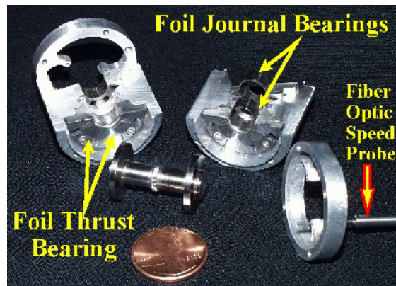
Fig. 1. Mesoscopic turbojet simulator rotor, split housing and MiTi ® split air foil bearings.
