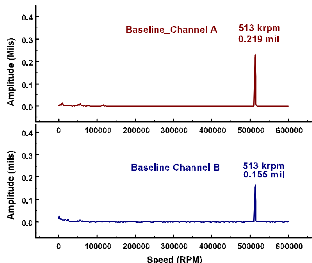
Fig. 9. Rotor vibration at 513,000 rpm for horizontal orientation.
