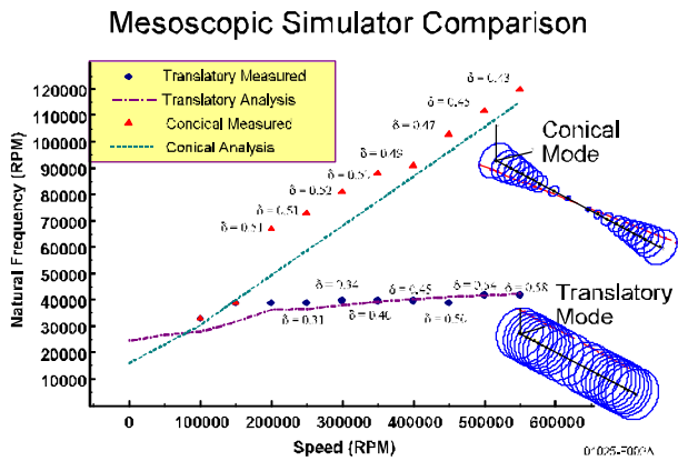
Fig 6. Whirl speed map and mode shapes for the mesoscopic rotor-bearing simulator system.
