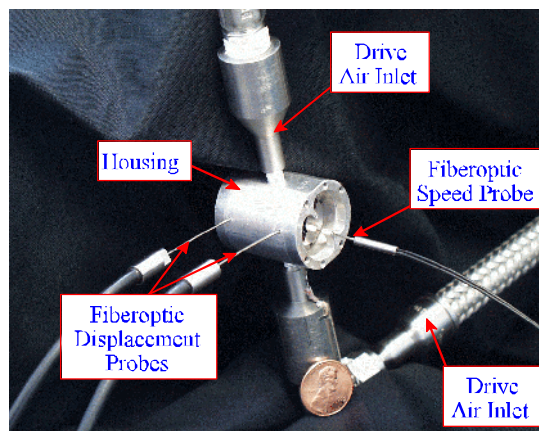
Fig. 2. Assembled and instrumented mesoscopic simulator.
