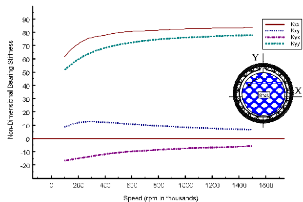
Fig. 5. Stiffness coefficients as a function of rotor speed for 6 mm diameter foil bearing .
