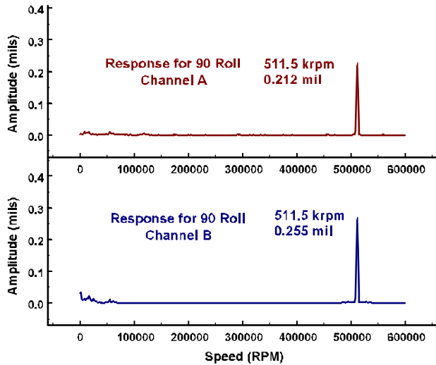
Fig. 10. Spectrum for 90° roll about spin axis.
