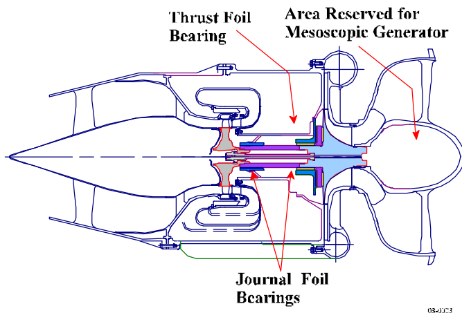
Fig. 3. Conceptual cross section diagram of oil-free mesoscopic turbojet engine.
