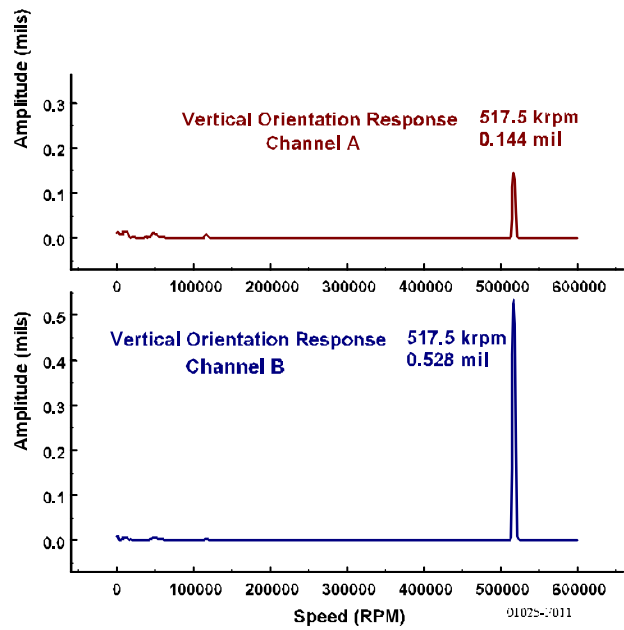
Fig. 12. Spectrum for vertical operation
