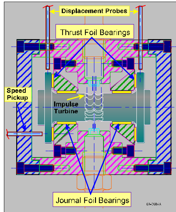
Fig. 4. Cross section of dynamic simulator.
